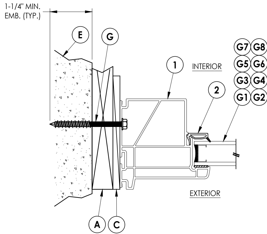
2 HORIZONTAL CROSS SECTION 2 Shown w/ 1X buck
