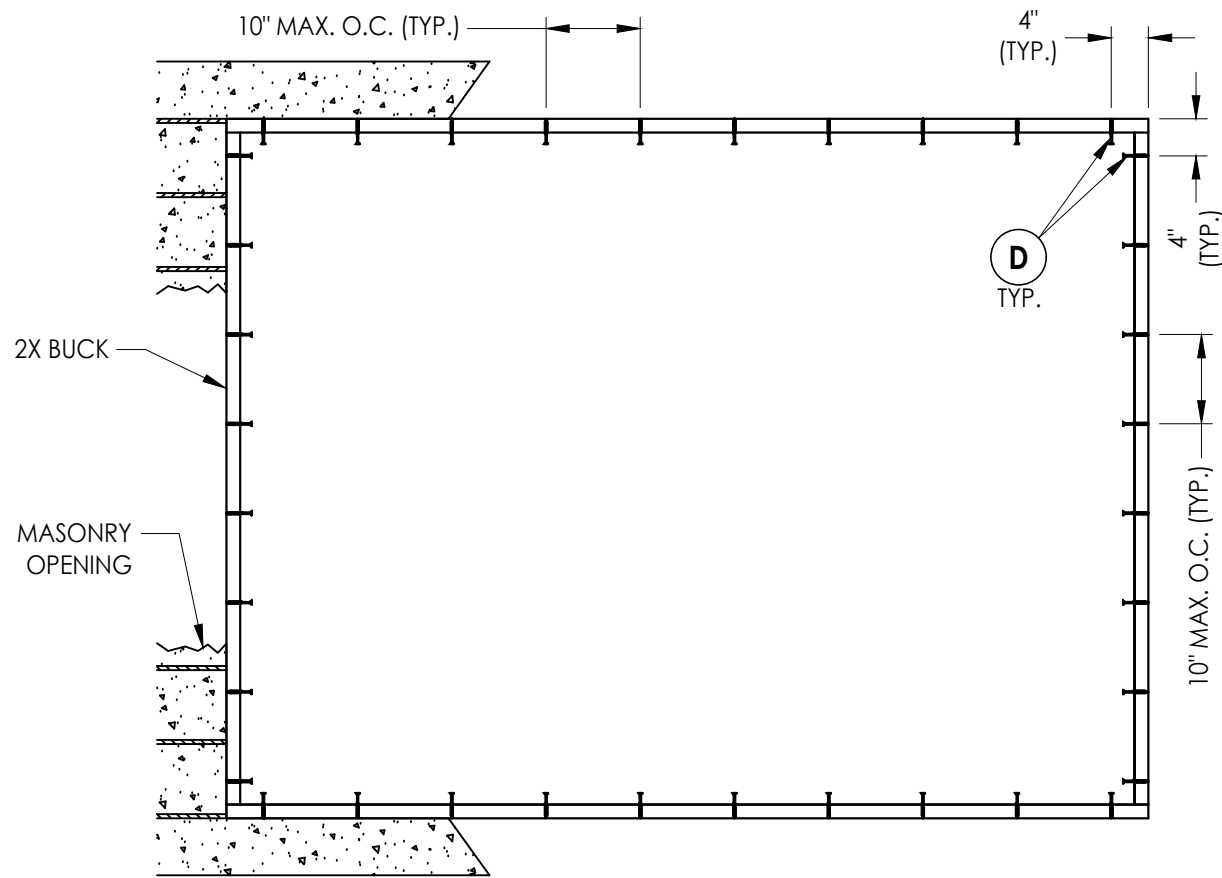
BUCK ANCHORING
