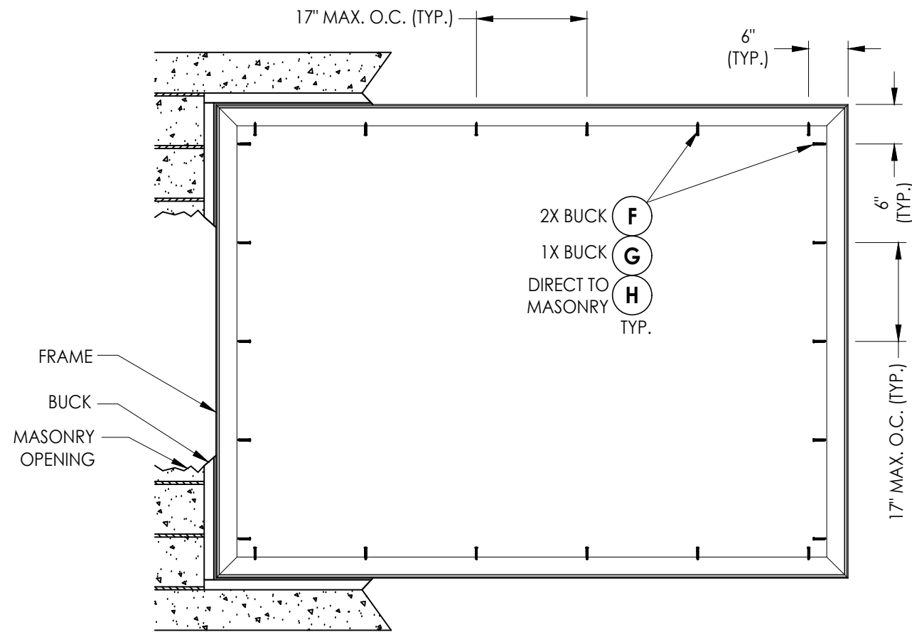
FRAME ANCHORING
